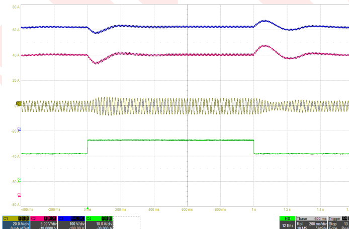
Figure 5: Load transient with 600 \mu\text{F} hold-up capacitor (50%-75%-50% of I_{max} , 115Vrms, 60Hz) Ch1: I_{in} (20A/div), Ch2: V_{out} (5V/div), Ch3: Hold-up capacitor voltage (100V/div), Ch4: I_{out} (10A/div), Timebase: (200ms/div).
