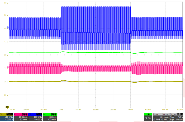
Figure 8: Input transient with 600µF hold-up capacitor at full load (115Vrms-220Vrms-115Vrms, 400Hz) Ch1: Vout (5V/div), Ch2: Iin (20A/div), Ch3: Vin (200V/div), Ch4: Vhold-up (100V/div), Timebase: (100ms/div).
