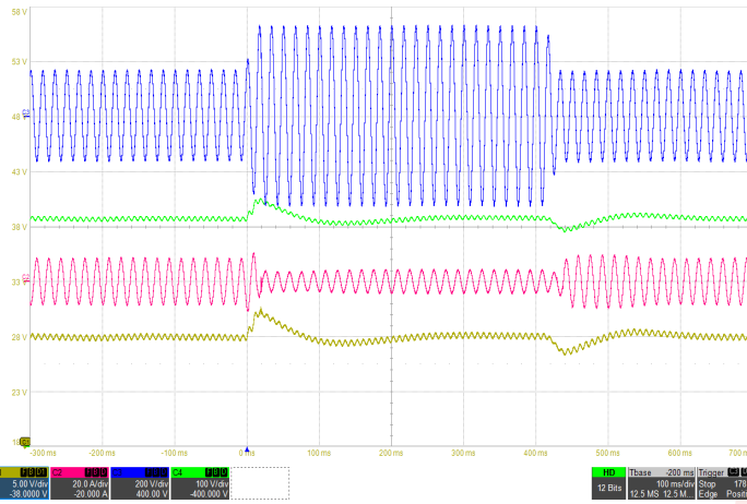
Figure 7: Input transient with 600µF hold-up capacitor at full load (115Vrms-220Vrms-115Vrms, 60Hz) Ch1: Vout (5V/div), Ch2: Iin (20A/div), Ch3: Vin (200V/div), Ch4: Vhold-up (100V/div), Timebase: (100ms/div).
