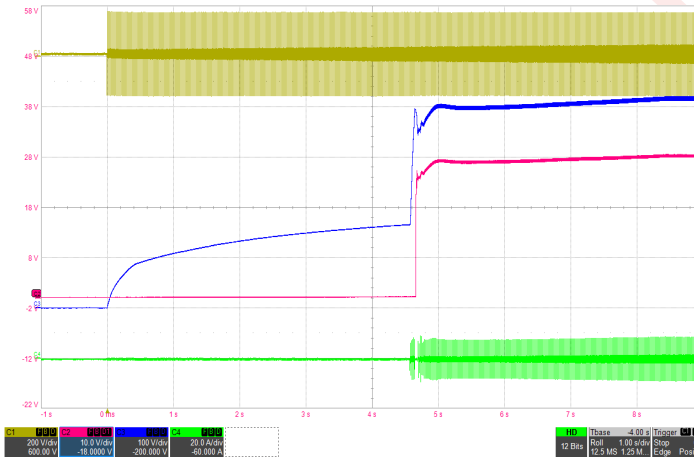
Figure 3: Typical startup waveform with 600 \mu\text{F} hold-up capacitor (115Vrms, 60Hz) Ch1: V_{in} (200V/div), Ch2: V_{out} (10V/div), Ch3: Hold-up capacitor voltage (100V/div), Ch4: I_{in} (20A/div), Timebase: (1s/div).
