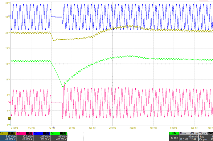
Figure 9: Line drop out with 600µF hold-up capacitor at full load (115Vrms, 60Hz) Ch1: Vout (5V/div), Ch2: Iin (10A/div), Ch3: Vin (200V/div), Ch4: Vhold-up (100V/div), Timebase: (100ms/div).
